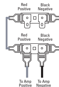
Figure 2. Connecting two woofers in parallel to the amplifier (2 ohms)
